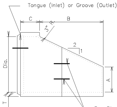
SIDE VIEW (SEE STANDARD PLATE 450.18 (TIE BOLTS FOR R.C.P. AND R.C.P. ARCH))
