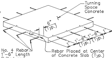
DETAIL E ISOMETRIC VIEW
