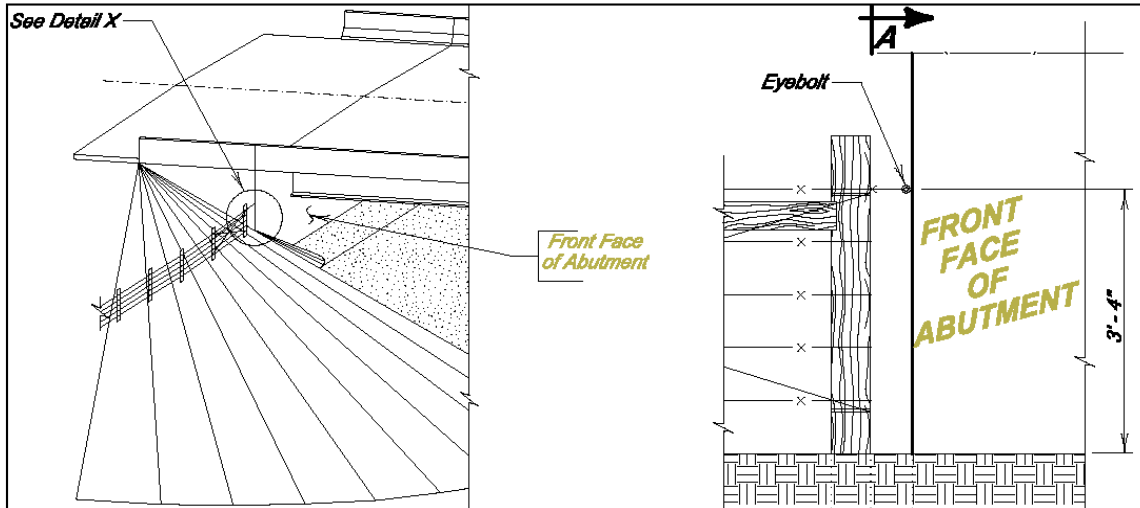
DETAIL "X"
