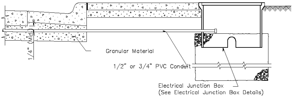
LEAD-IN DETAIL
