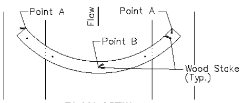
PLAN VIEW DITCH INSTALLATION
