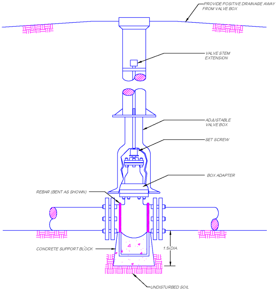
GATE VALVE & BOX NOT TO SCALE
