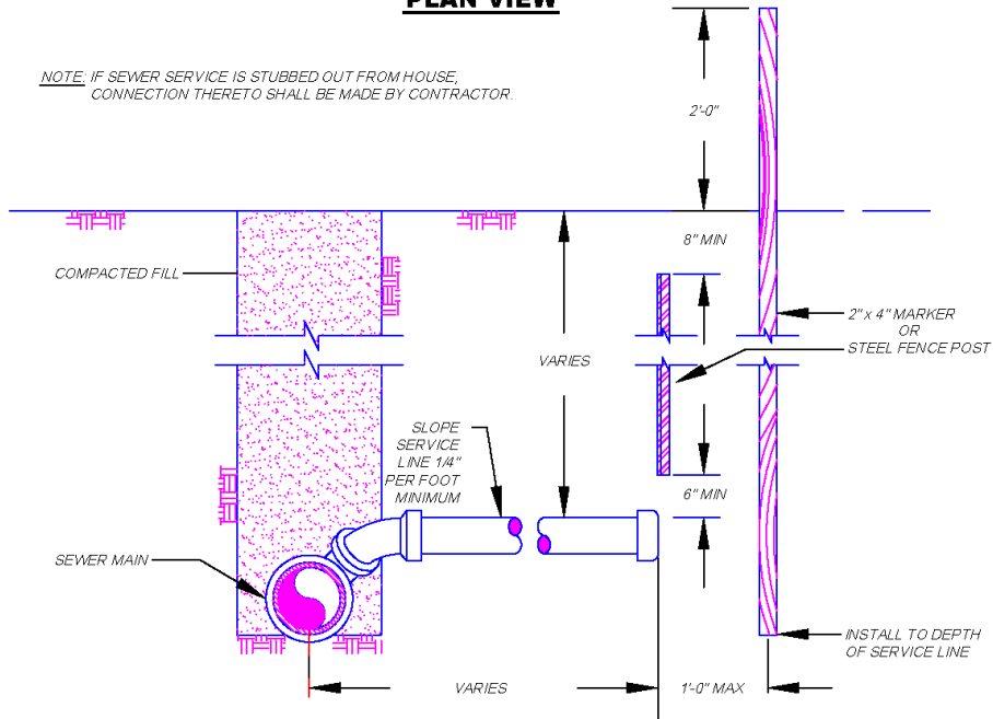
PROFILE VIEW
