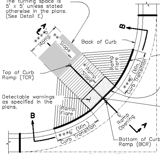
PLAN VIEW (With 6'+ Curb Transition)
