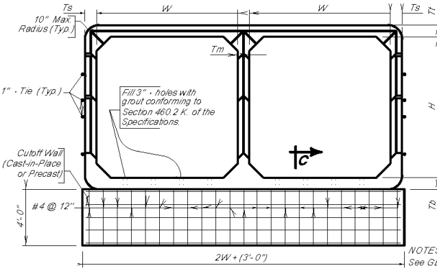
VIEW A - A
