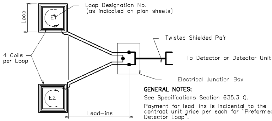
WIRING DIAGRAM
