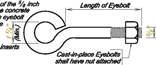
EYEBOLT DETAILS
