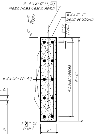
SEC. C - C
