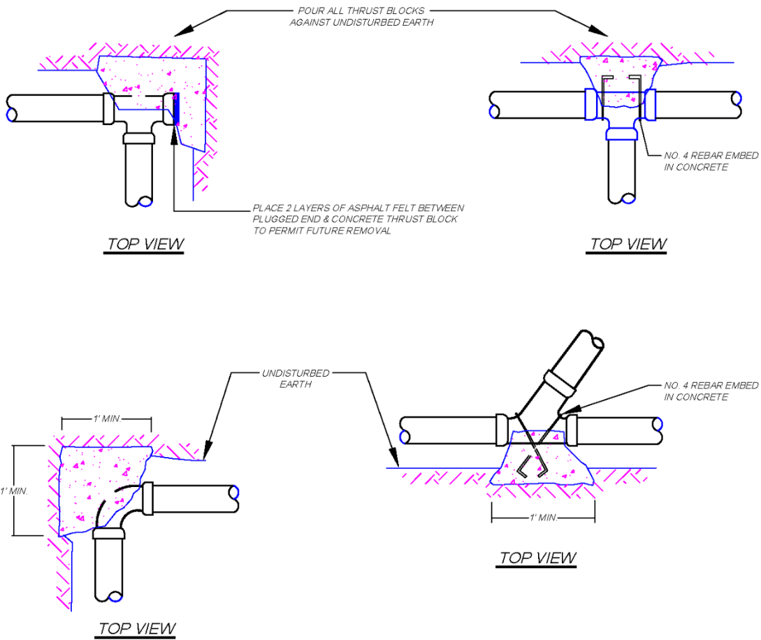
THRUST BLOCK SETTINGS NOT TO SCALE
