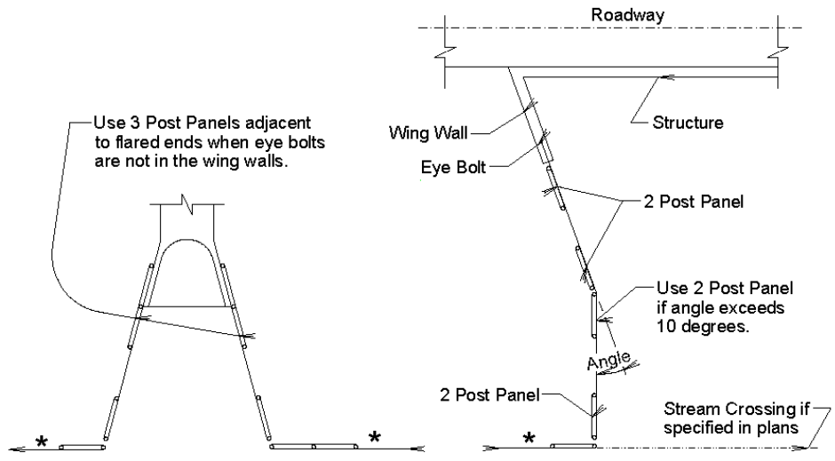
R.C. BOX CULVERT OR CATTLE PASS
