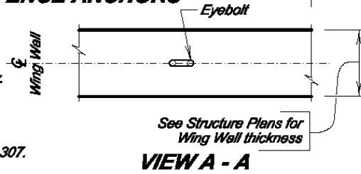
DETAIL FOR FENCE ANCHORS
