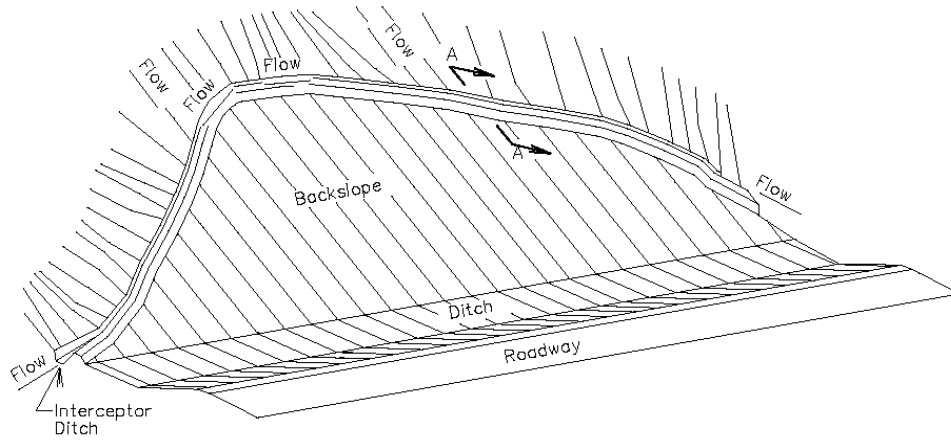
ISOMETRIC VIEW
