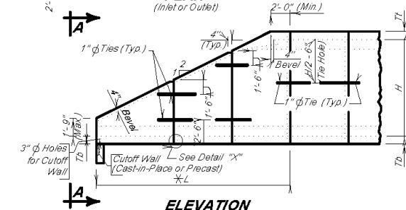
ELEVATION (Inlet or Outlet)
