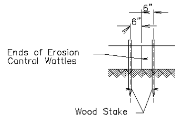
DETAIL C
