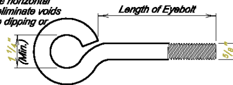
EYEBOLT DETAILS
