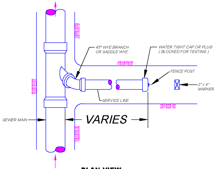
PLAN VIEW
