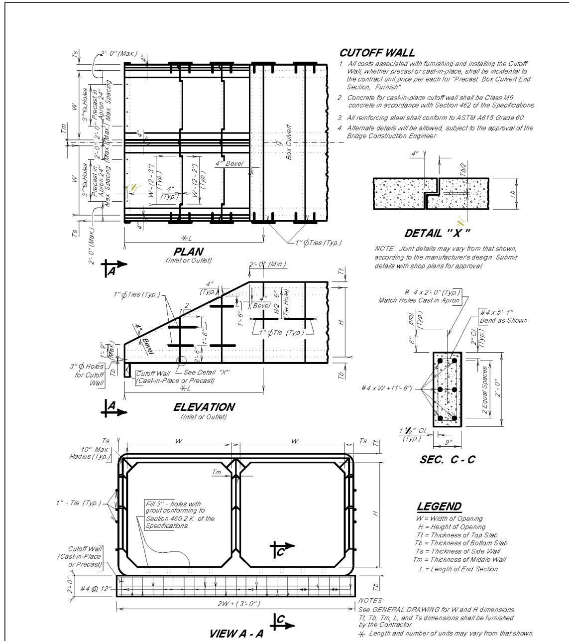
PRECAST DOUBLE BOX CULVERT WITH SLOPED END (2' CUTOFF WALL) NOT TO SCALE
