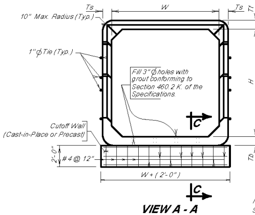
PRECAST BOX CULVERT WITH SLOPED END SECTION NOT TO SCALE
