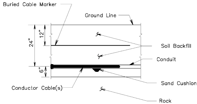
SECTION VIEW
