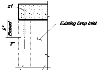
SEC. C - C
