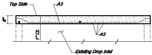
SEC. A - A
