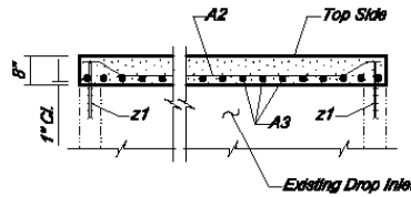
SEC. B - B
