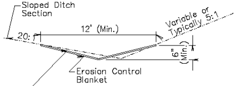
STANDARD DITCH SECTION
