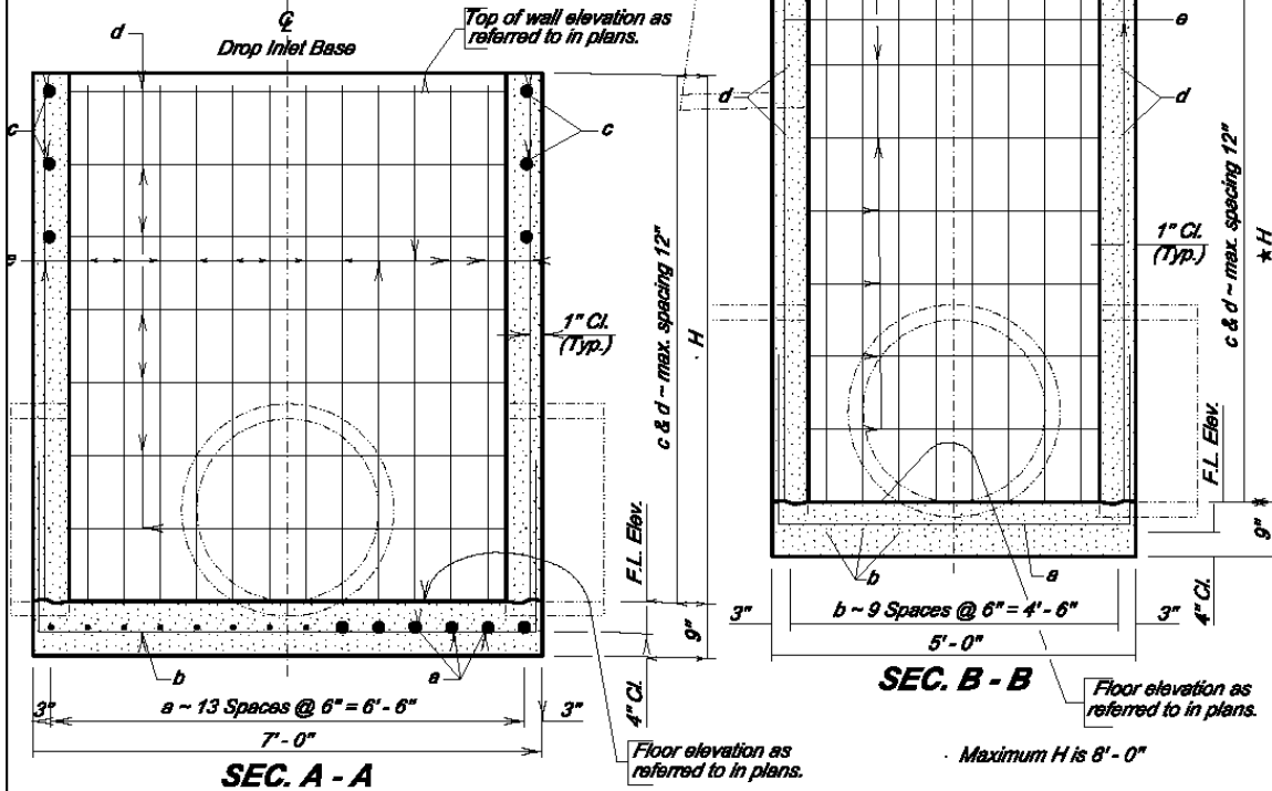
DROP INLET-CONCRETE-TYPE S (4'X6') NOT TO SCALE
