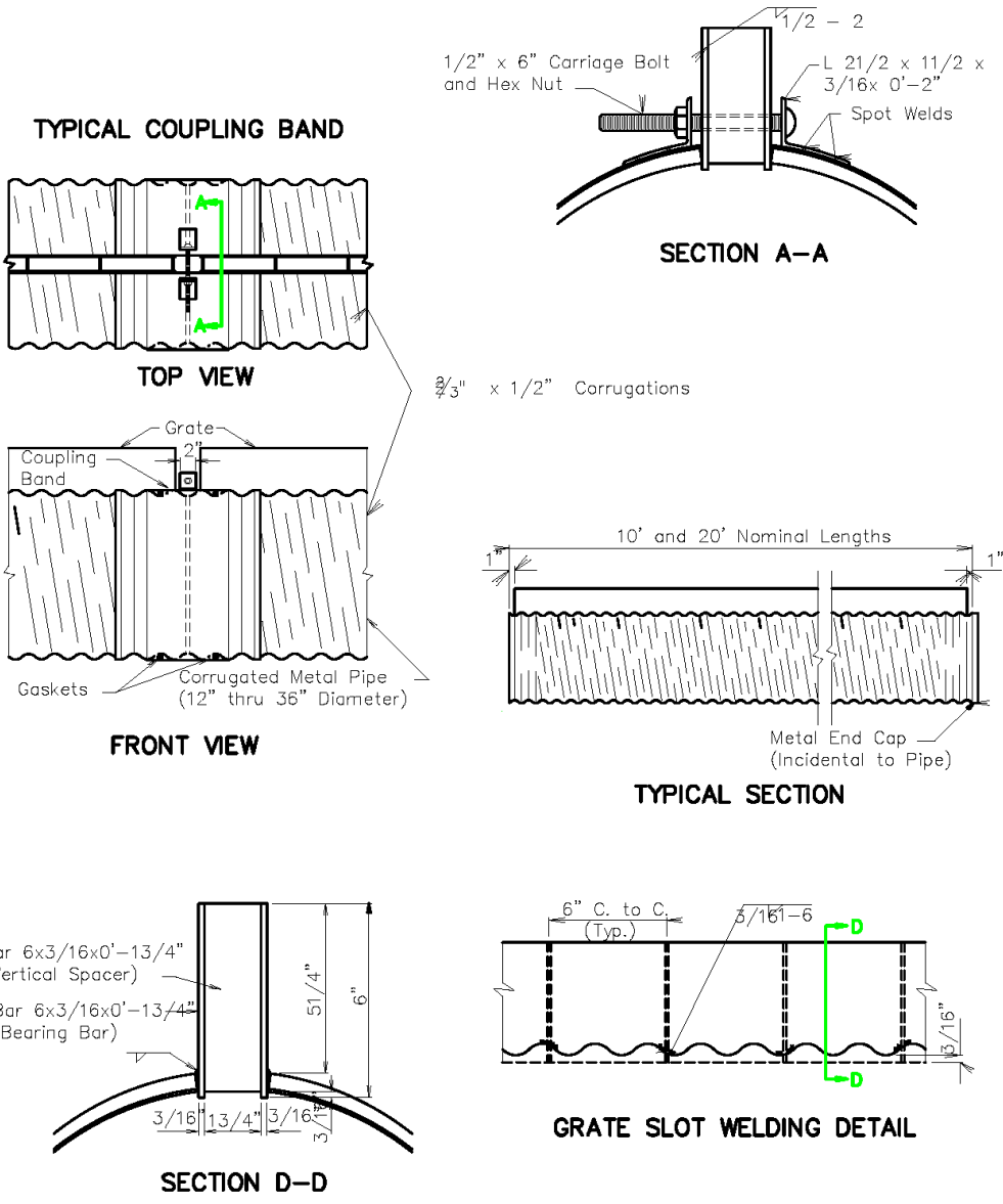
CORRUGATED METAL PIPE SLOTTED DRAIN-1 NOT TO SCALE
