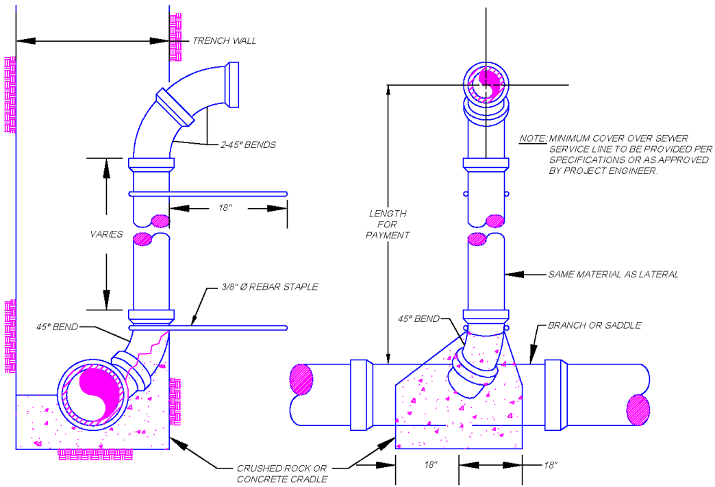
SEWER SERVICE RISER NOT TO SCALE
