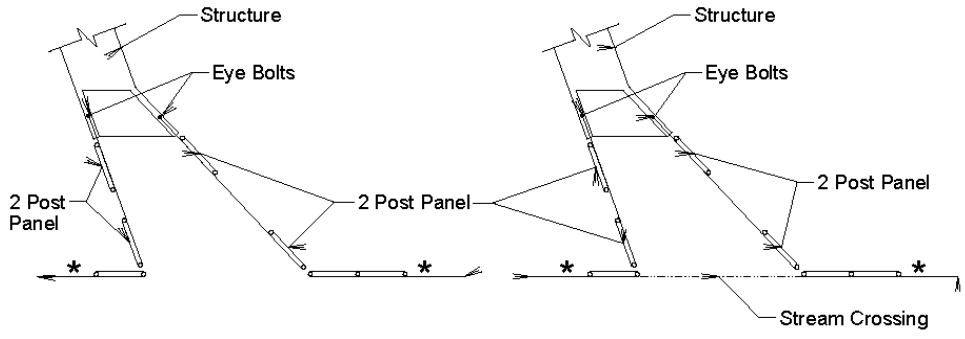
R.C. BOX CULVERT OR CATTLE PASS
