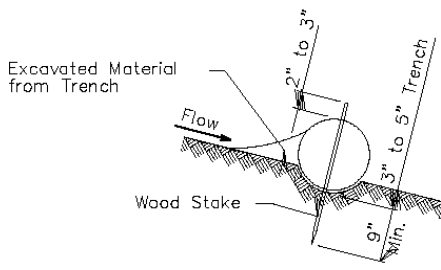
DETAIL B (TYPICAL OF ALL INSTALLATIONS)
