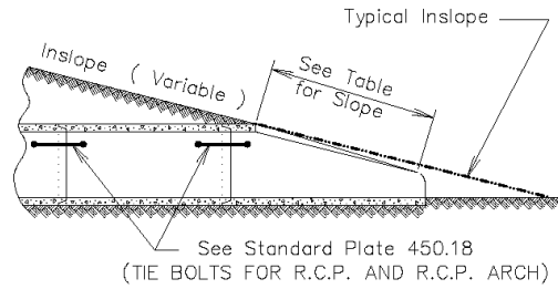
SLOPE DETAIL
