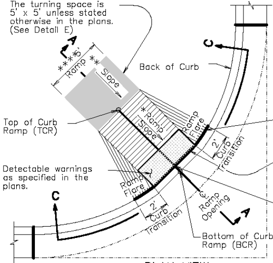
PLAN VIEW (With 2' Curb Transition)
