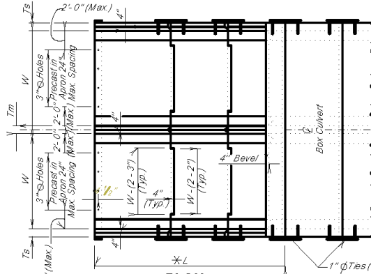
PLAN (Inlet or Outlet)
