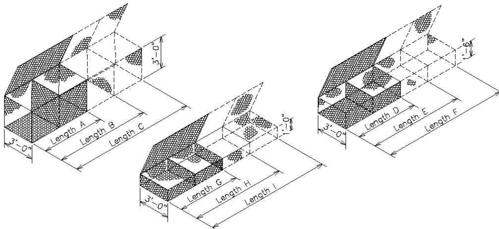
GABION DETAILS STANDARD SIZES
