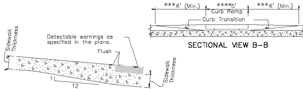
DETAIL D
