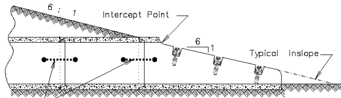
ELEVATION VIEW
